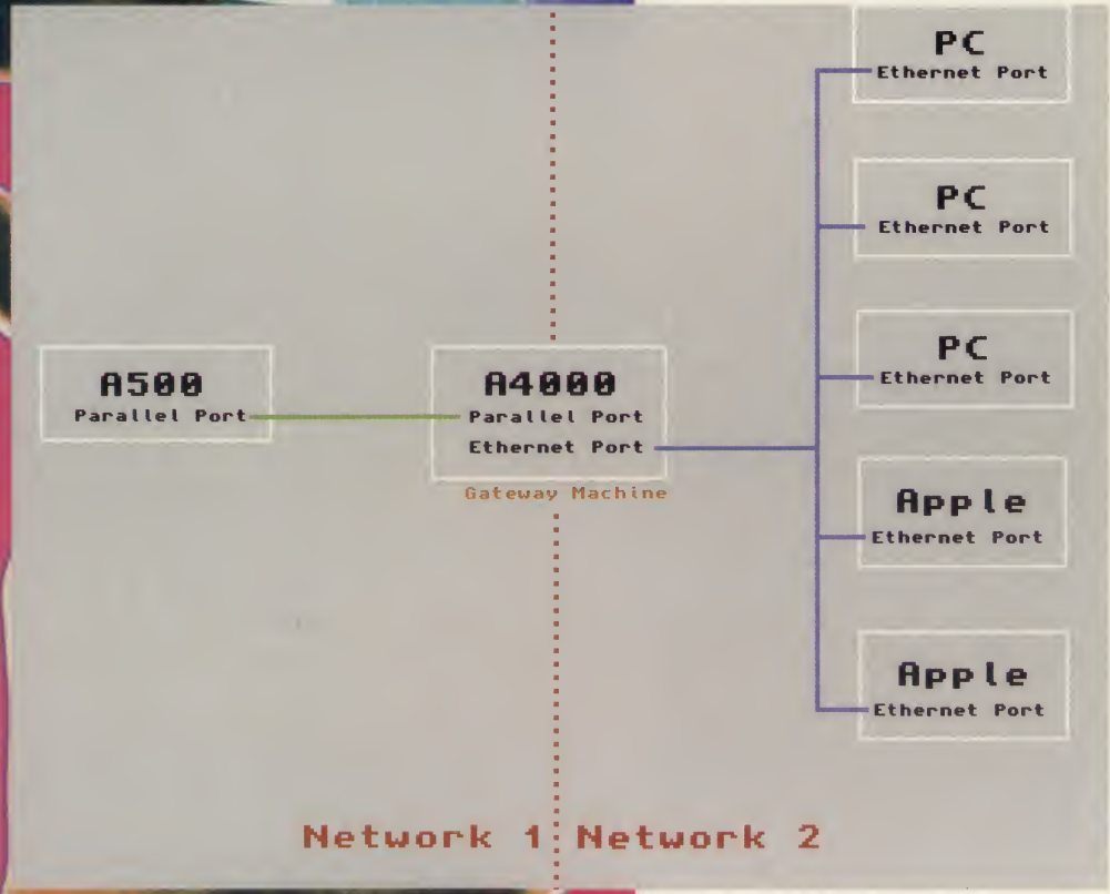
LEFT: Here's how an A500 can be networked to a LAN full of PCs or Apples. The A4000 has an Ethernet card and acts as a gateway between the two networks. The technical term for this set-up is an "internet" with a small "i".
